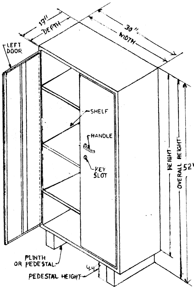
SKETCH OF STEEL SHELVING CABINET
